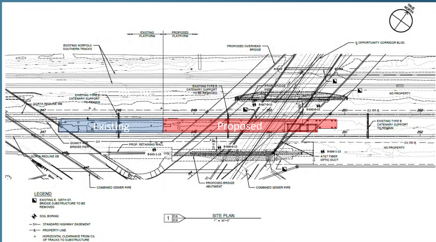
Site Plan
