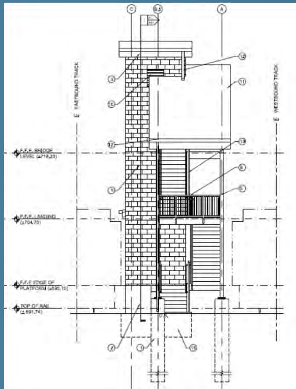
East Elevation
