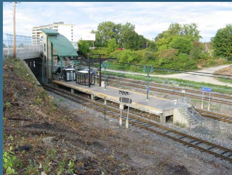
Existing Station – Platform Level
