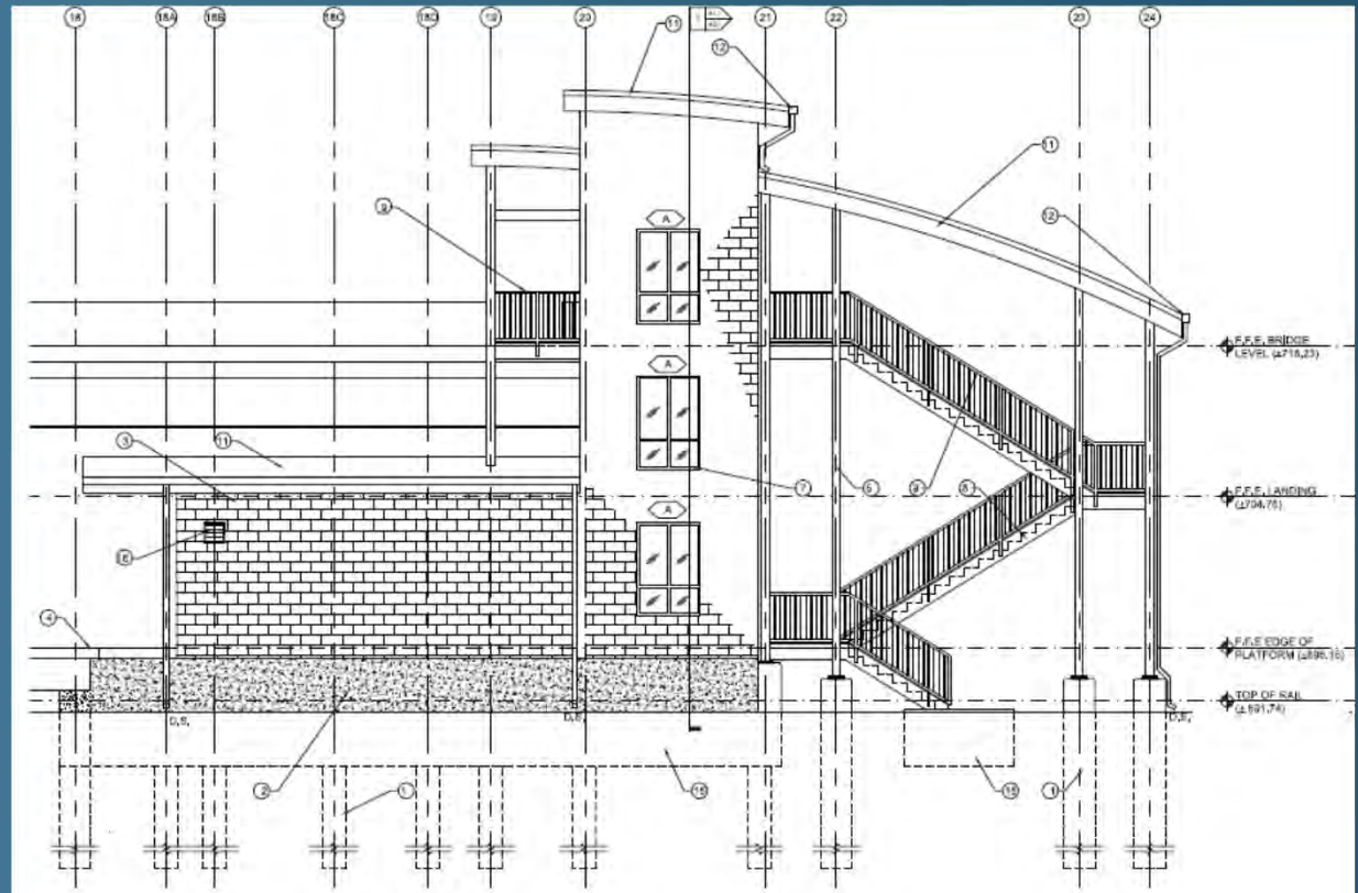
South Elevation
